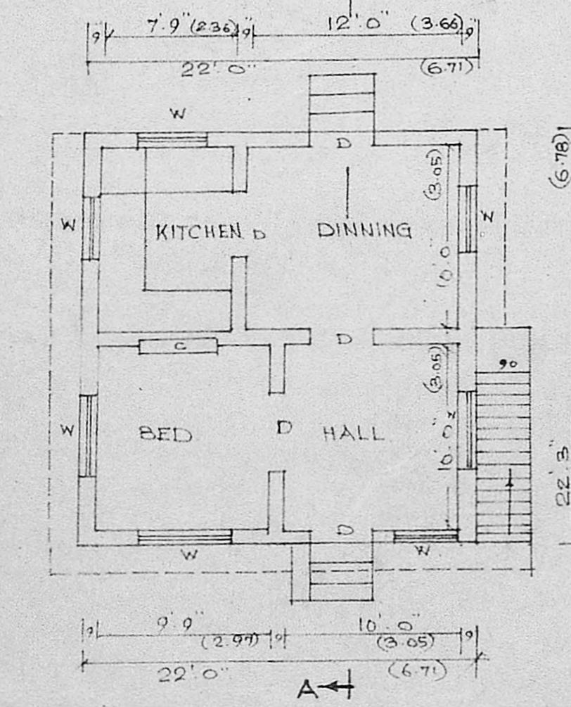
PLAN OF G. FLOOR.
