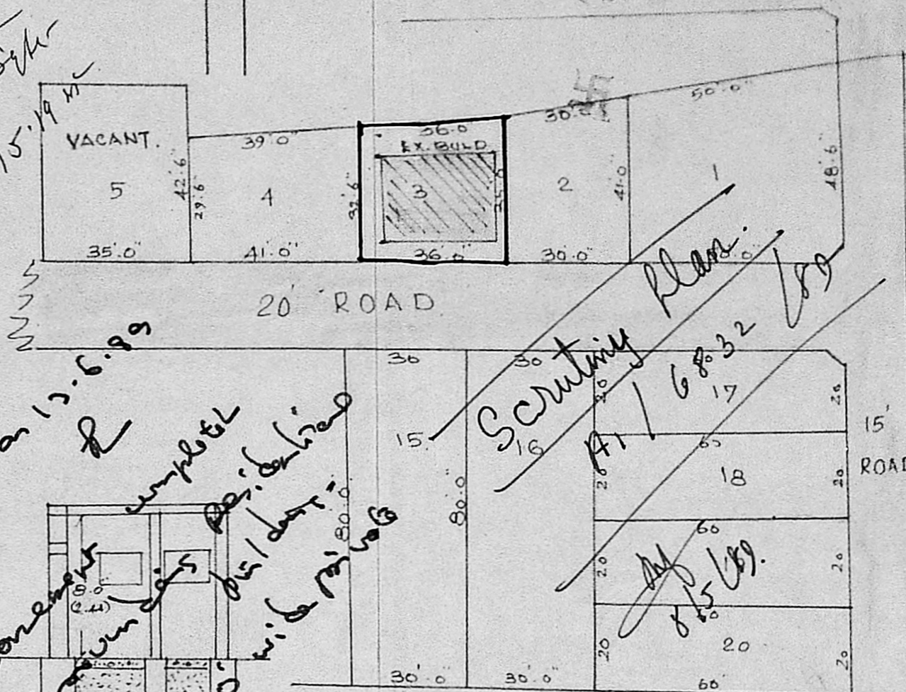
PT OF LAY-OUT. SCALE 1 INCH - 33 FEET.
